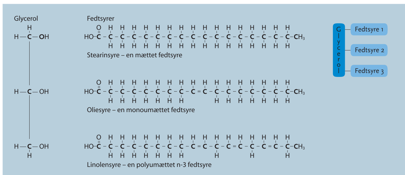
Figur 42. Triglycerid (fedtstof).
